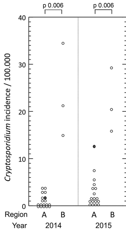
Fig. 1. Each dot represents an incidence of Cryptosporidium per 100 000 people within a single county. The calculated mean incidence of Cryptosporidium in the 18 Swedish counties (Region A) in comparison with the mean incidence in the Uppsala, Halland and Jönköping counties (Region B) in 2014 and 2015. One county has been marked with a grey dot; they introduced PCR-based screening including Cryptosporidium of all faecal samples in June 2015.
